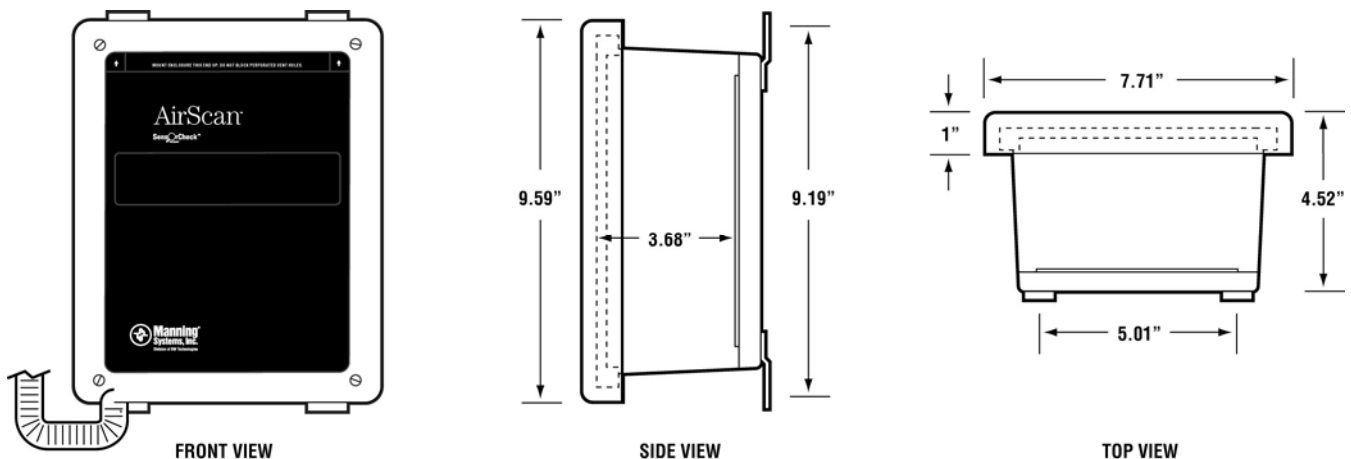
Figure 1: Mounting Dimensions
